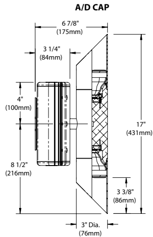
CAMLOCK CANOPY
